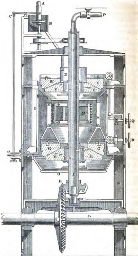
WESTRUP'S CONICAL MILL.
